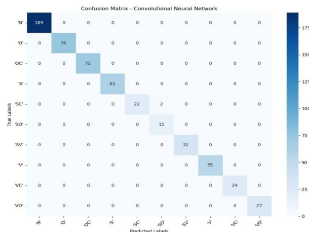
Figure 9: Overall results of the CNN model
