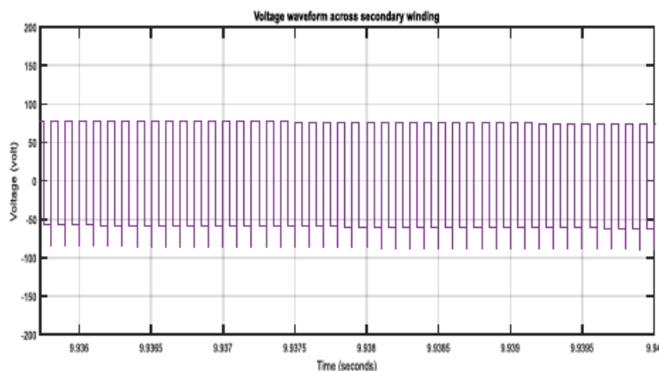
Fig -4: Secondary coil voltage waveform
