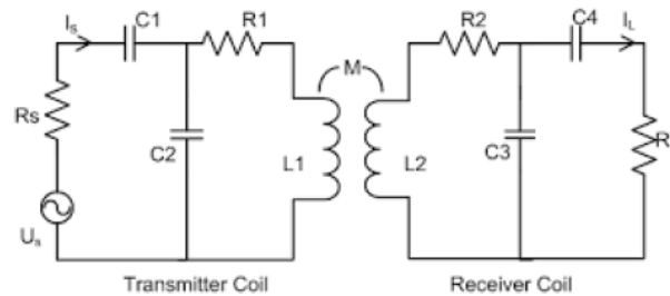
Figure 1: Model circuit of WPT system
