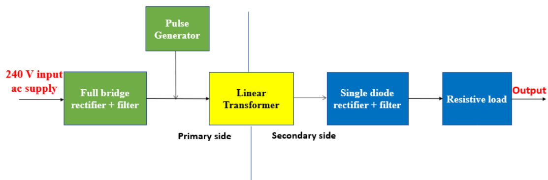
Fig -2: Block diagram of MATLAB simulated circuit of wireless power transfer system
