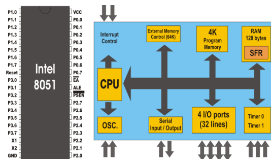
Figure 2: The Intel Microcontroller architecture
