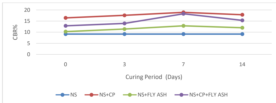
Figure 12: Variation of Soaked CBR with Curing Period
