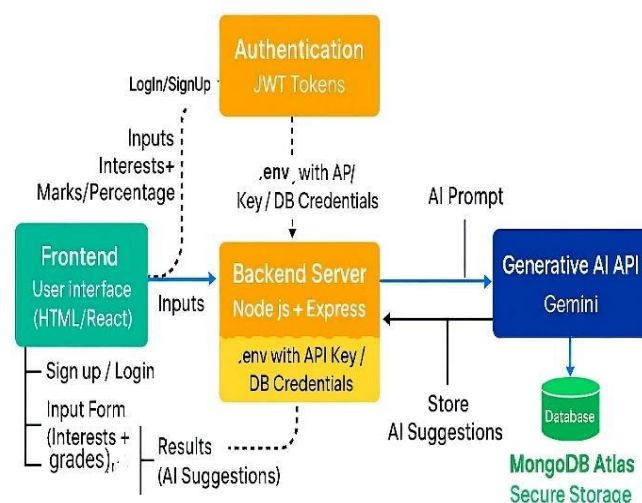
Figure 1: Block Diagram of AI-Based Career Guidance System
